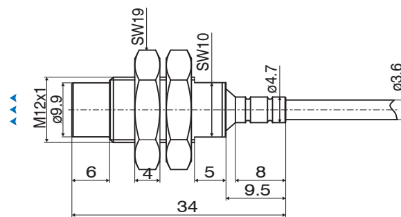
Fig. 5 ES-U3-C-CAx, dimensions in mm (not to scale)
