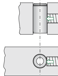
Mounting with grub screw (plastic)
