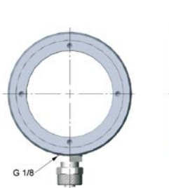
TM-W-CTL Water cooled housing
