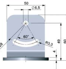
TM-FB-CTL Mounting bracket (fixed); included in CTL scope of supply
